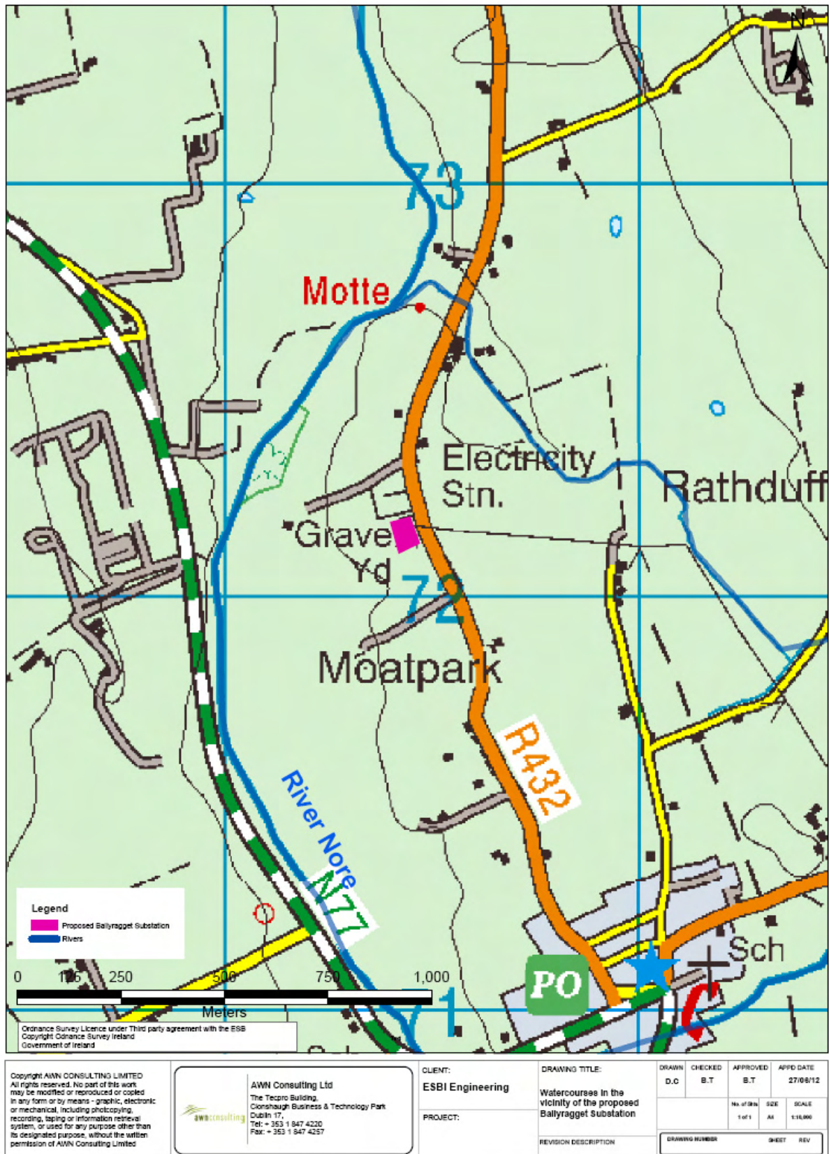
Figure 10.6 Watercourses in the vicinity of the proposed Ballyragget Substation
