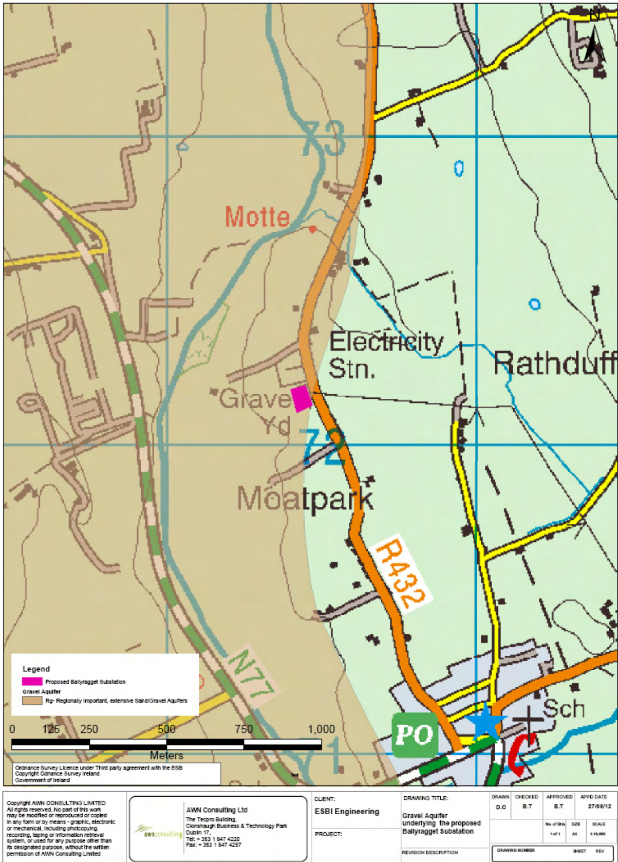
Figure 10.8 Gravel Aquifers underlying the proposed Ballyragget Substation
