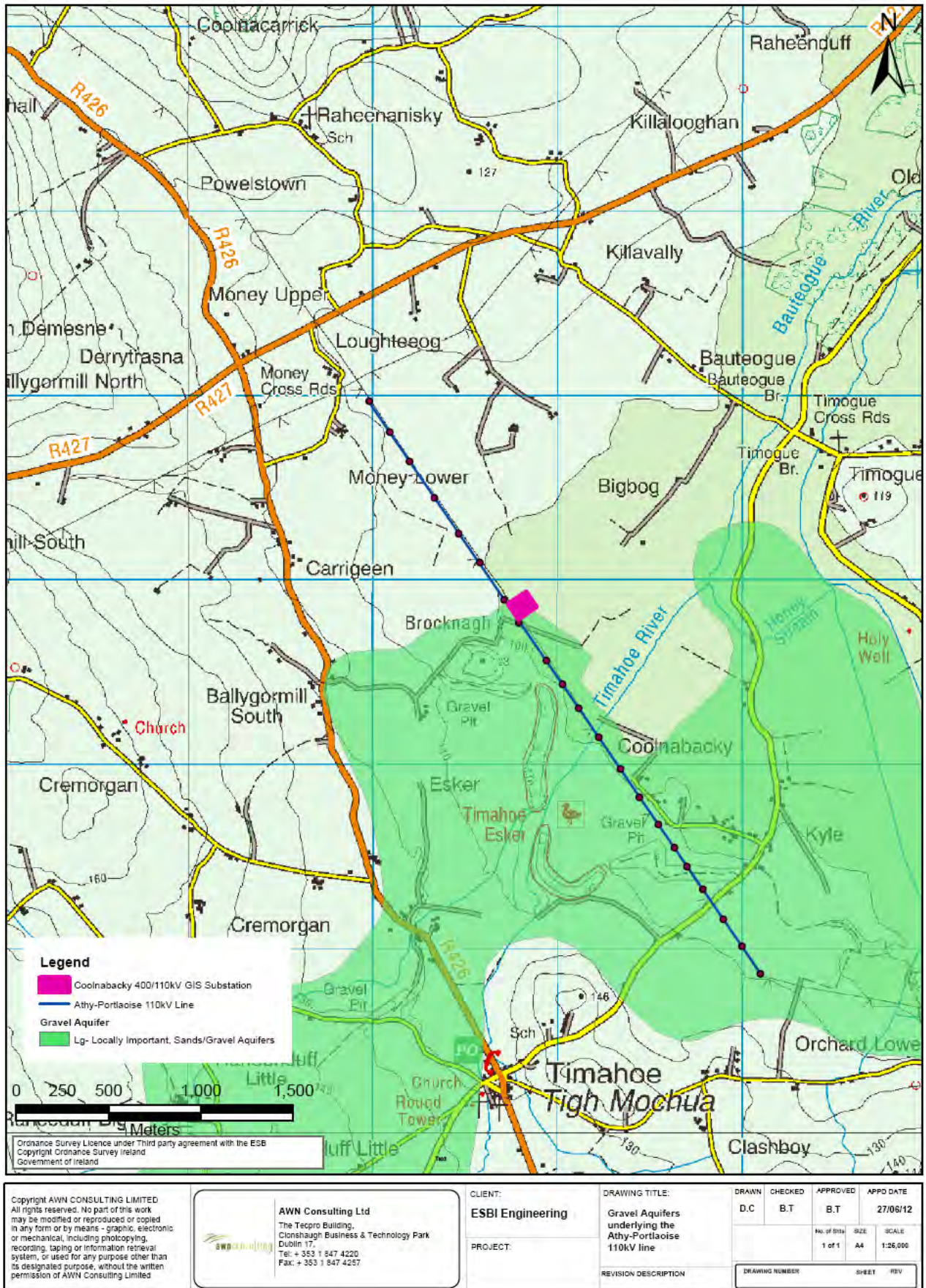
Figure 10.28 Gravel Aquifers underlying the Athy-Portlaoise 110kV line
