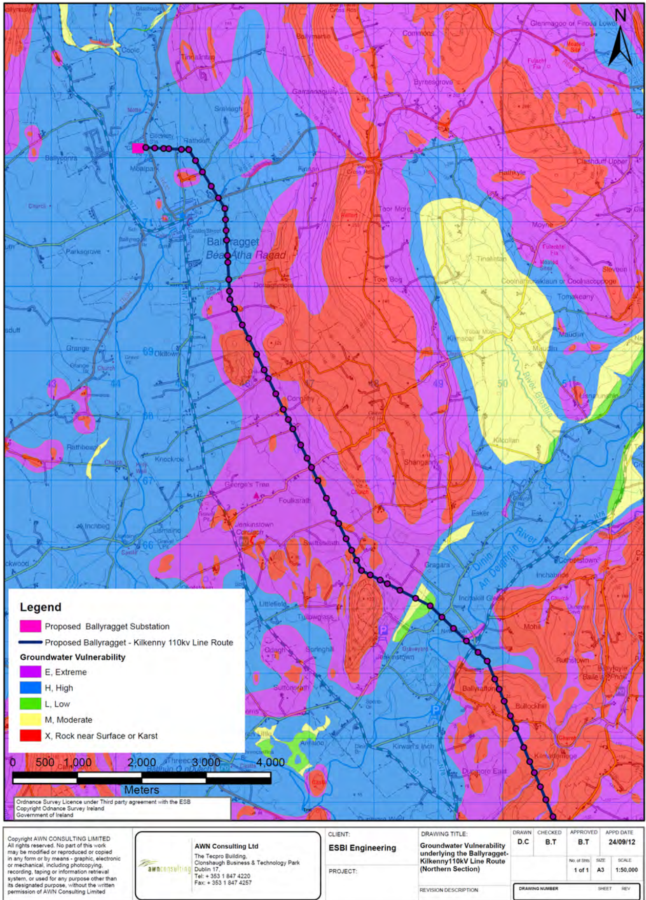
Figure 10.24 Groundwater Vulnerability underlying the Ballyragget – Kilkenny 110kv Line Route (Northern Section)
