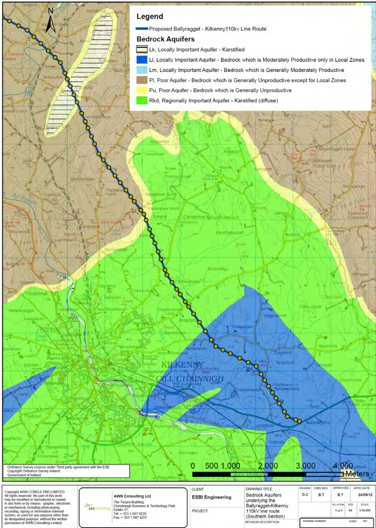
Figure 10.21 Bedrock Aquifers underlying the Ballyragget – Kilkenny 110kV Line Route (Southern Section)
