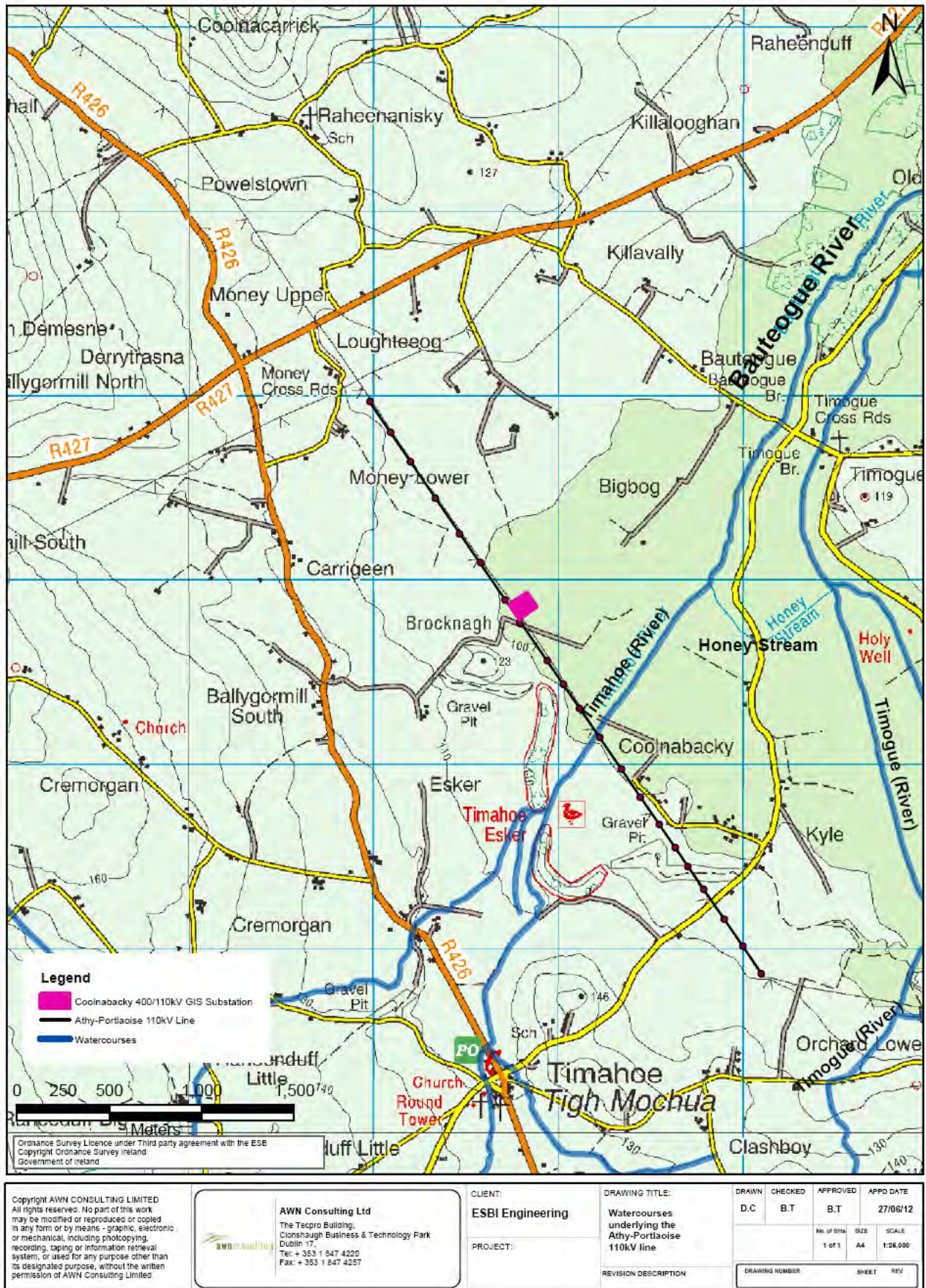
Figure 10.26 Watercourses in the vicinity of the Athy-Portlaoise 110kV line
