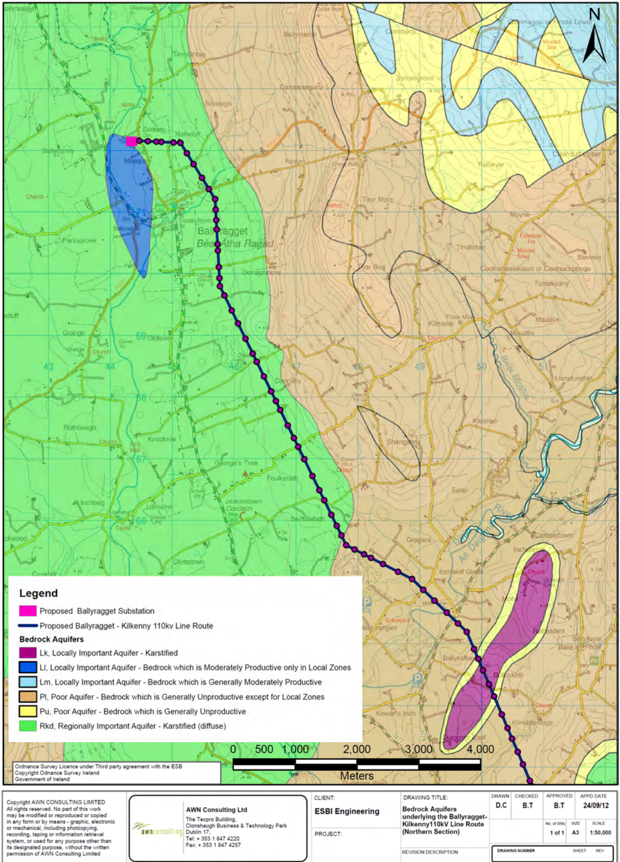
Figure 10.20 Bedrock Aquifers underlying the Ballyragget – Kilkenny 110kV Line Route (Northern Section)
