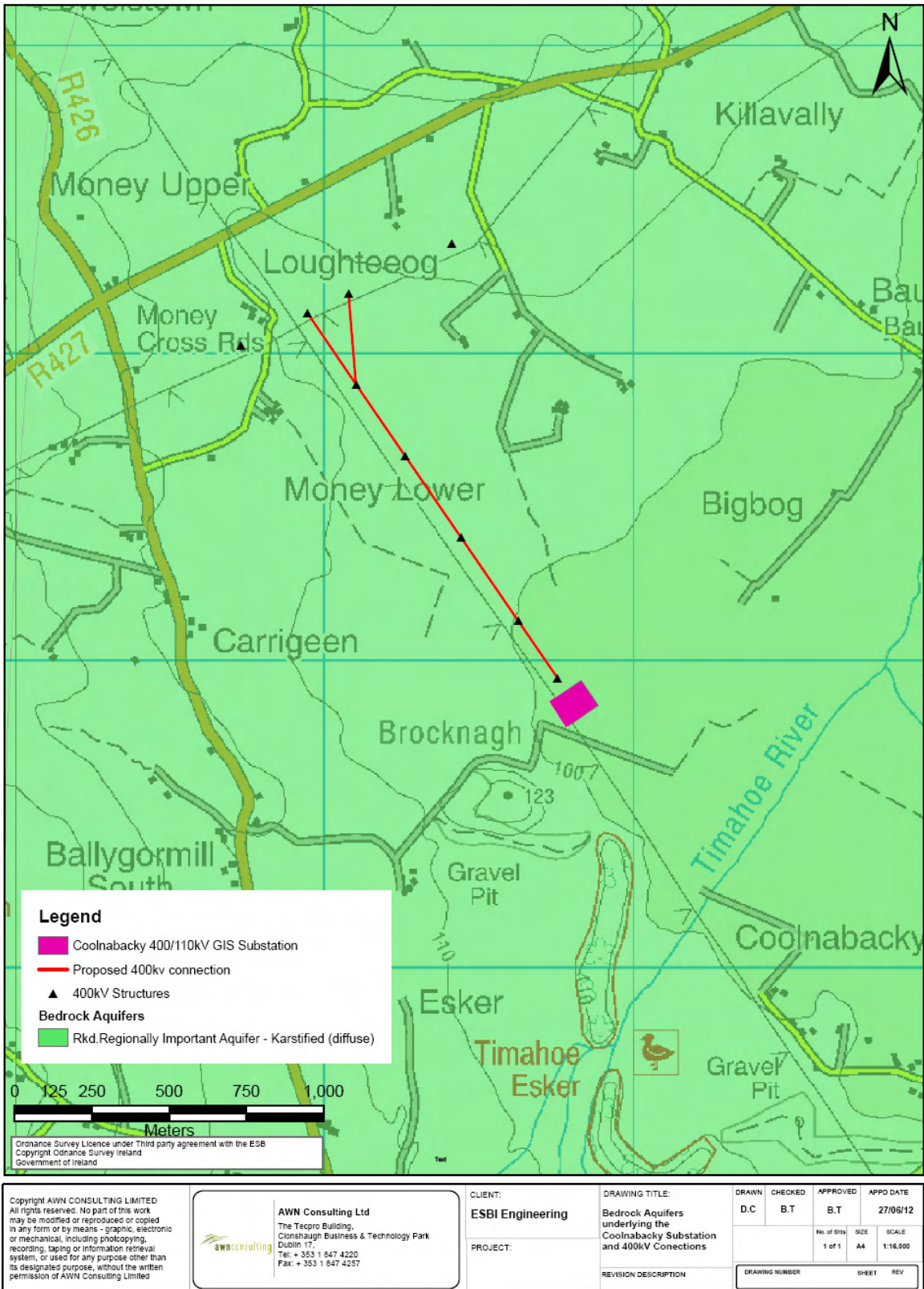
Figure 10.3 Bedrock Aquifers underlying the proposed Coolnabackey Substation and 400kV Connections
