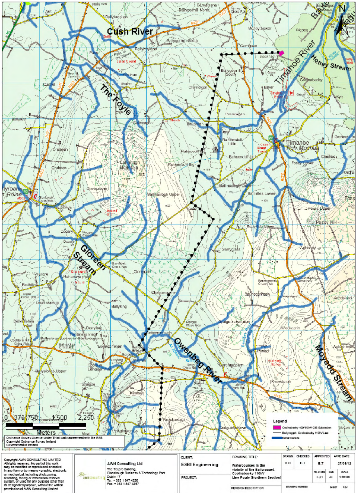
Figure 10.10 Watercourses in the vicinity of the proposed Ballyragget – Coolnabackey 110kV Line Route (Northern Section)
