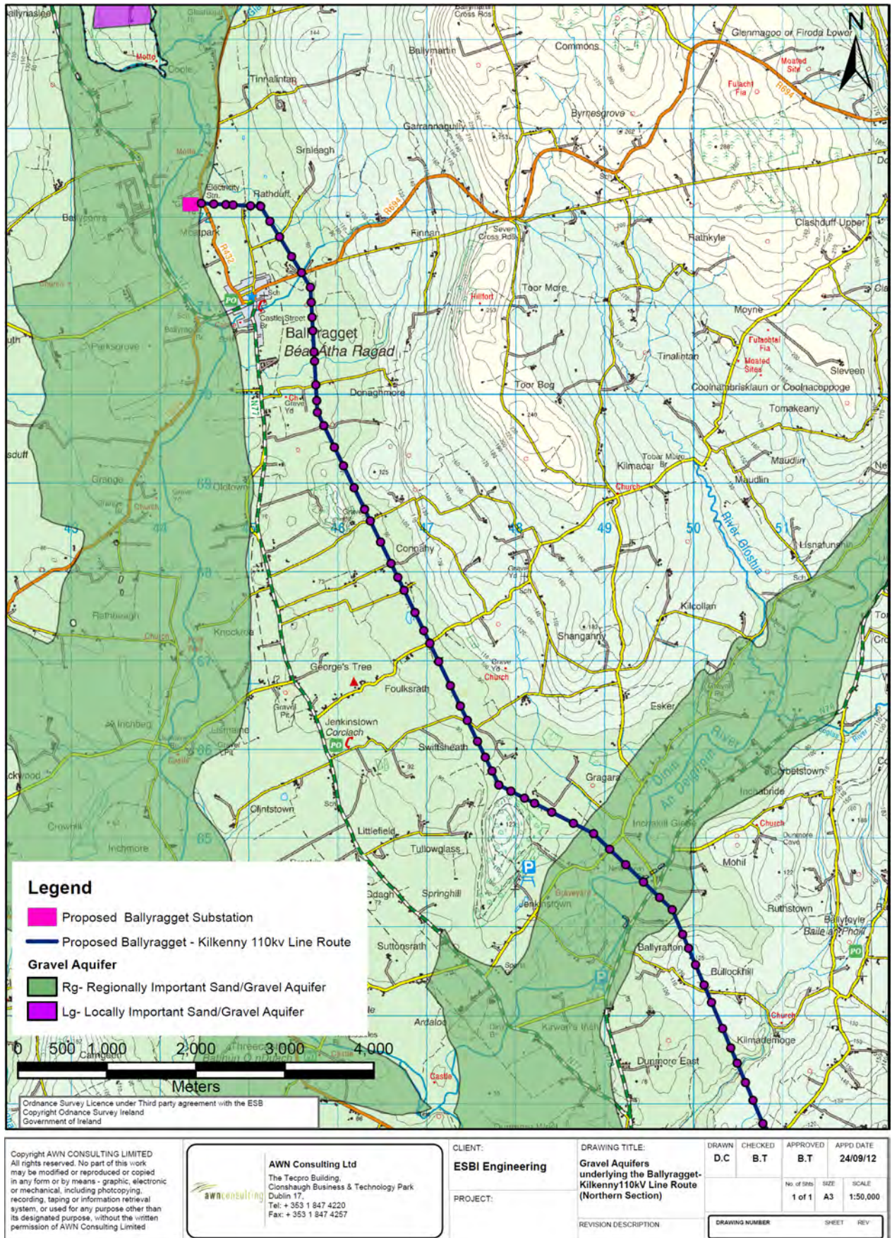
Figure 10.22 Gravel Aquifers underlying the Ballyragget – Kilkenny 110kV Line Route (Northern Section)
