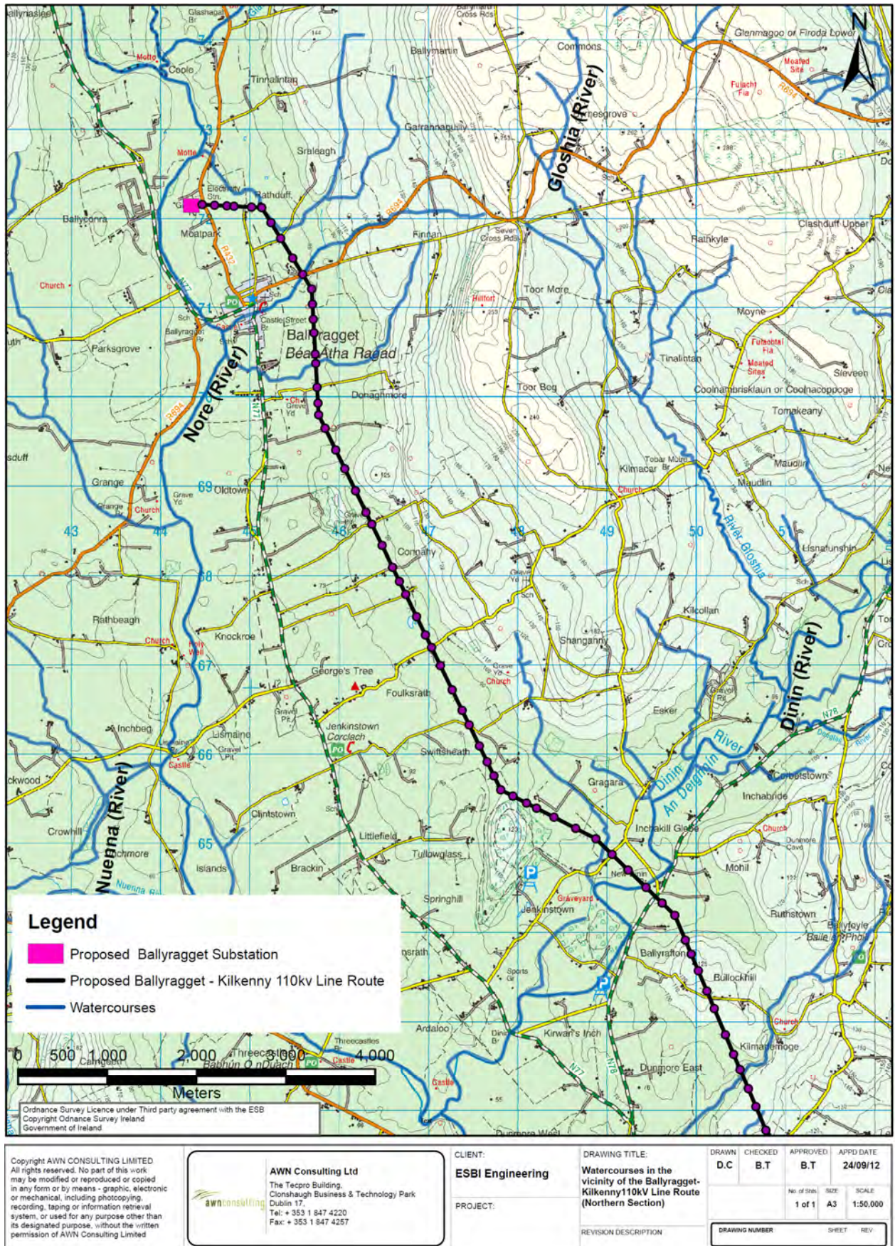
Figure 10.18 Watercourses in the vicinity of the Ballyragget – Kilkenny 110kV Line Route (Northern Section)
