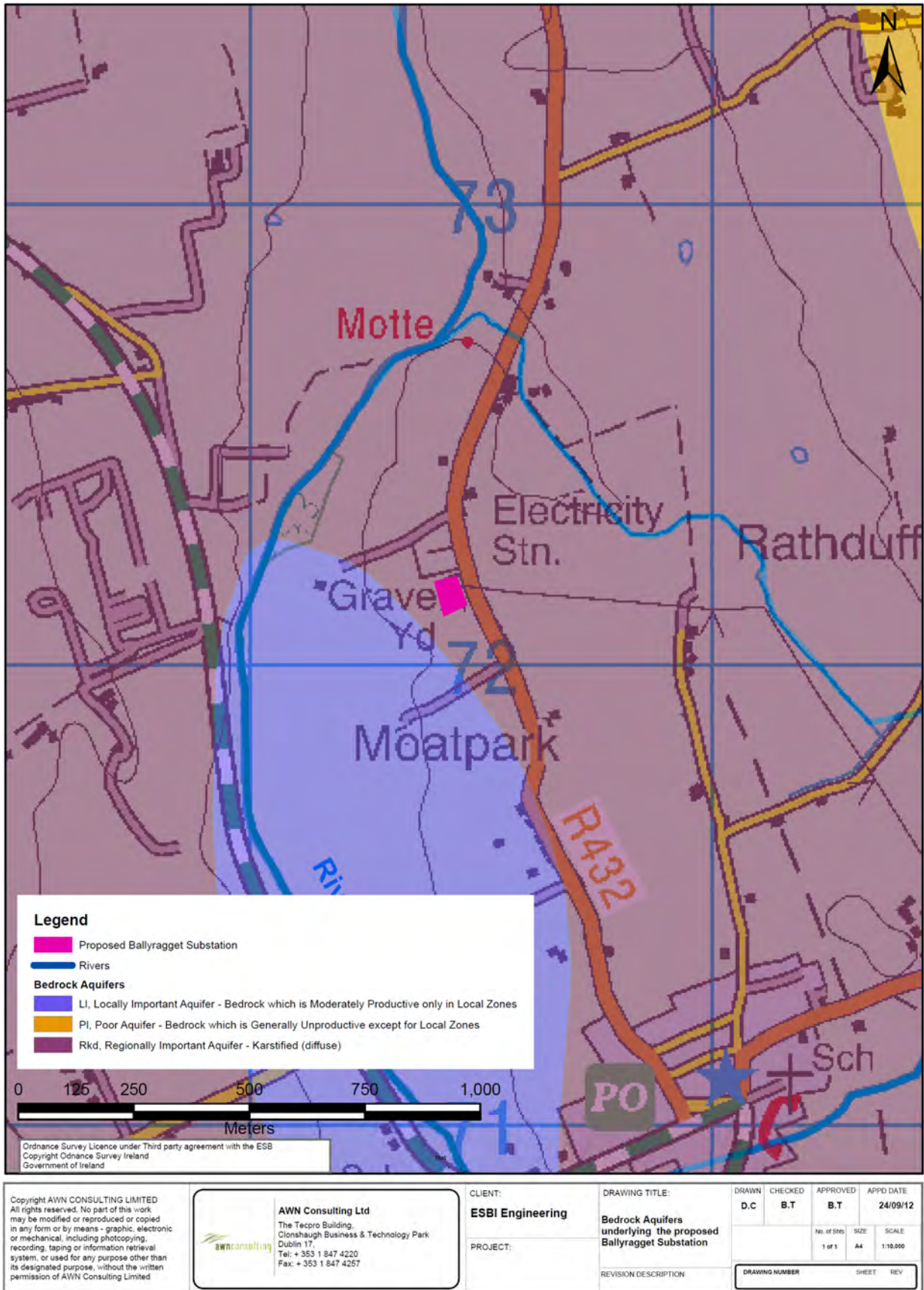
Figure 10.7 Bedrock Aquifers underlying the proposed Ballyragget Substation
