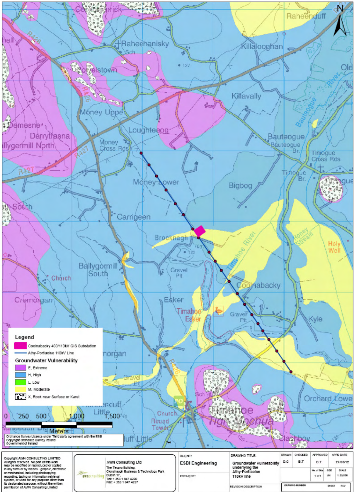
Figure 10.29 Groundwater Vulnerability underlying the Athy-Portlaoise 110kV line
